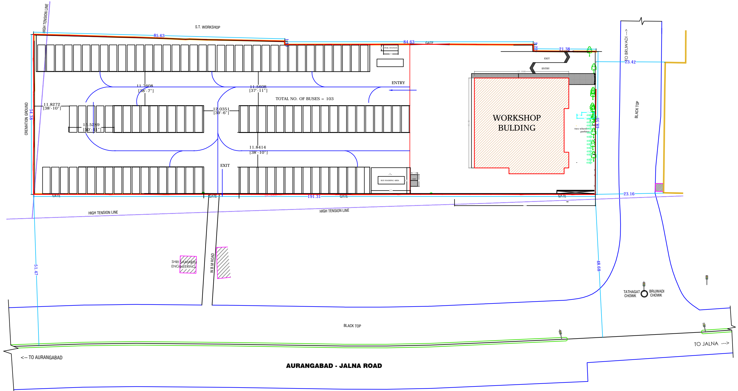
SITE PLAN (PARKING LAYOUT)
